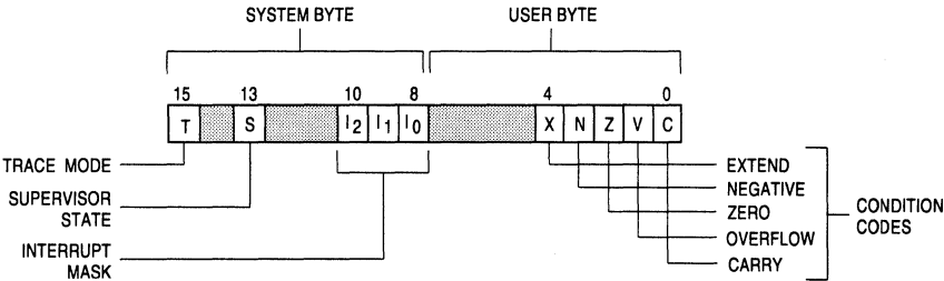
Figure 2-4. Status Register
